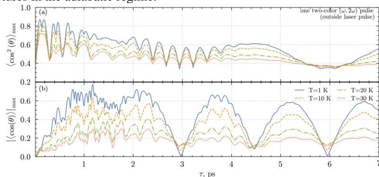
Fig. 1. The dependence of the maximum the degrees of alignment ( \langle \cos^2(\theta) \rangle_{\max} ) (a) and orientation ( |\langle \cos(\theta) \rangle|_{\max} ) (b) on the trapezoidal laser pulse duration \tau . The different temperatures T = 1, 10, 20, 30 K are indicated by a solid, dashed, dash-dotted and dotted lines respectively.
